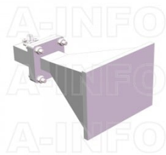
LB-90-15-C-3.5SPO Standard Gain Horn Antenna 8.2-12.4GHz 15dB Gain 3.5mm Female
